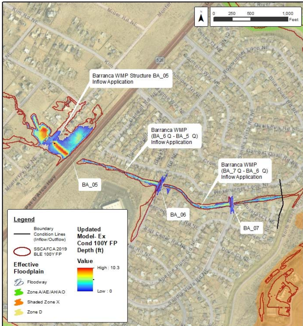
Figure 2.12: Flooding as a result of the 100-year storm in the vicinity of structures BA_05, BA_06 & BA_07 under existing conditions (tributary B).
