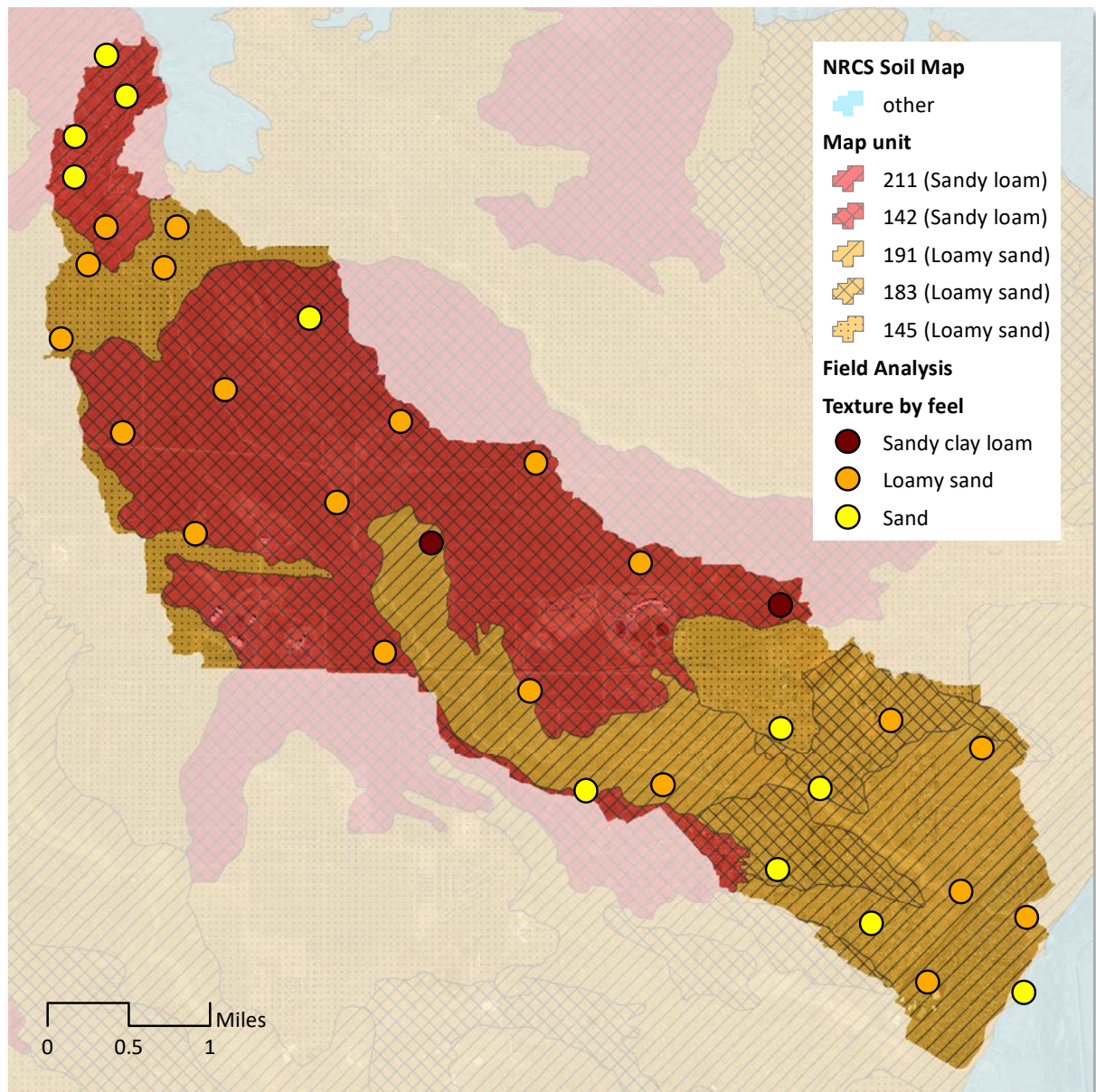
Figure 1.3: Near-surface soil textures found in the Barranca watershed based on NRCS soil map (shaded) and field assessment conducted by SSCAFCA at 33 sites (circles).
