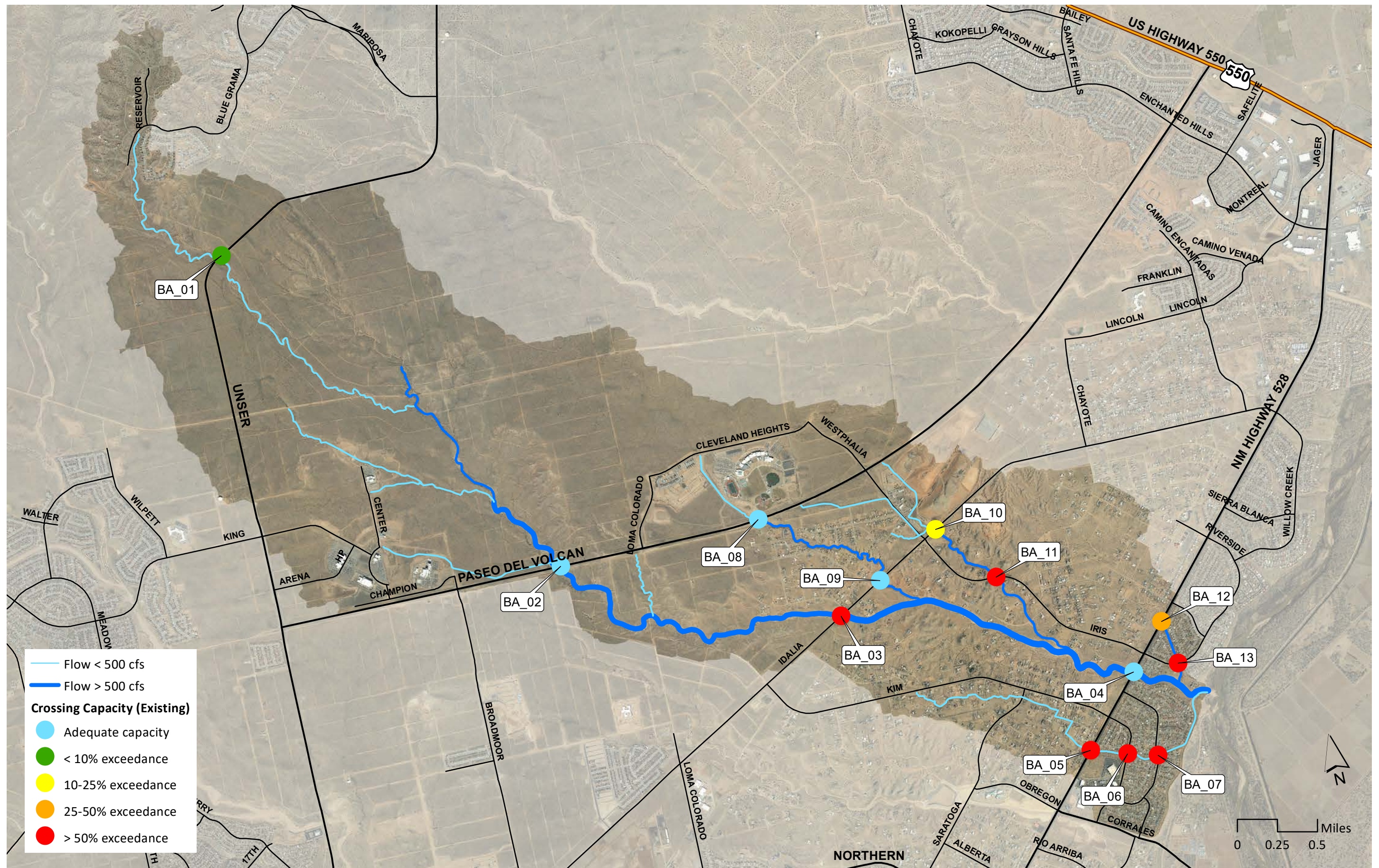
Figure 2.7: Major crossing structures and deficiencies in the Barranca watershed (Existing conditions).
