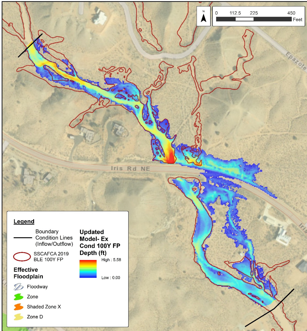
Figure 2.14: Flooding as a result of the 100-year storm in the vicinity of structure BA_11 under existing conditions (tributary H).
