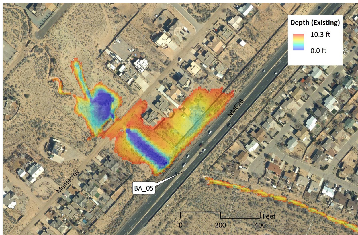
Figure 3.3: Crossing structure BA_11 in tributary B and extent of expected flooding during existing conditions.
